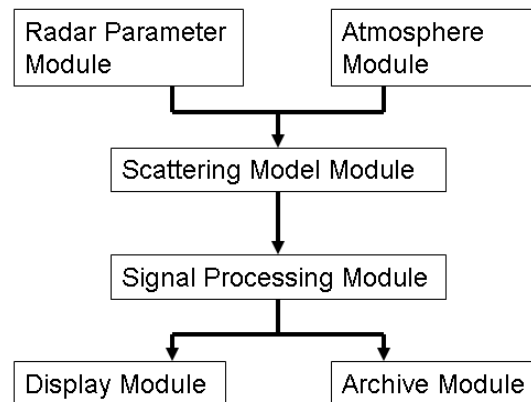
Figure 1. Flow diagram of the Radar Simulator.
