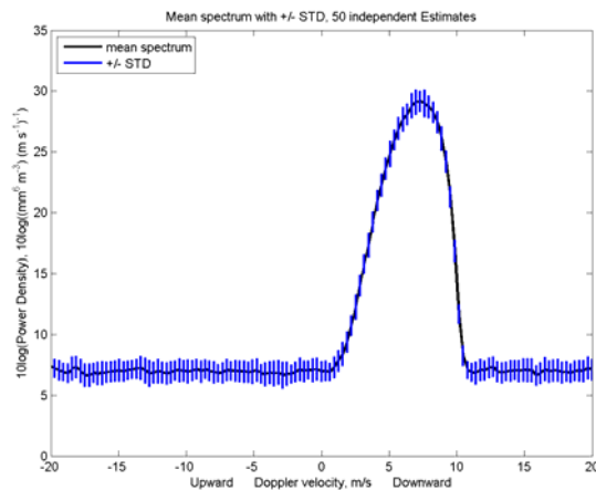
Figure 3. Mean reflectivity-weighted Doppler velocity power spectral density (black line) for 50 simulations. The input DSD parameters were Z = 30 dBZ, D_0 = 1.5 mm, \mu = 3 , and the air motion was zero with a spectrum broadening of 0.25 \text{ m s}^{-1} . Plus and minus one standard deviation at each Doppler velocity bin is shown with the blue lines. The standard deviation of the reflectivity from the 50 simulations was 0.41 dBZ.
