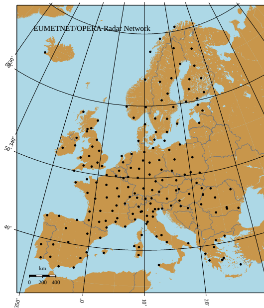
Figure 2. Map showing the weather radar network of OPERA.
