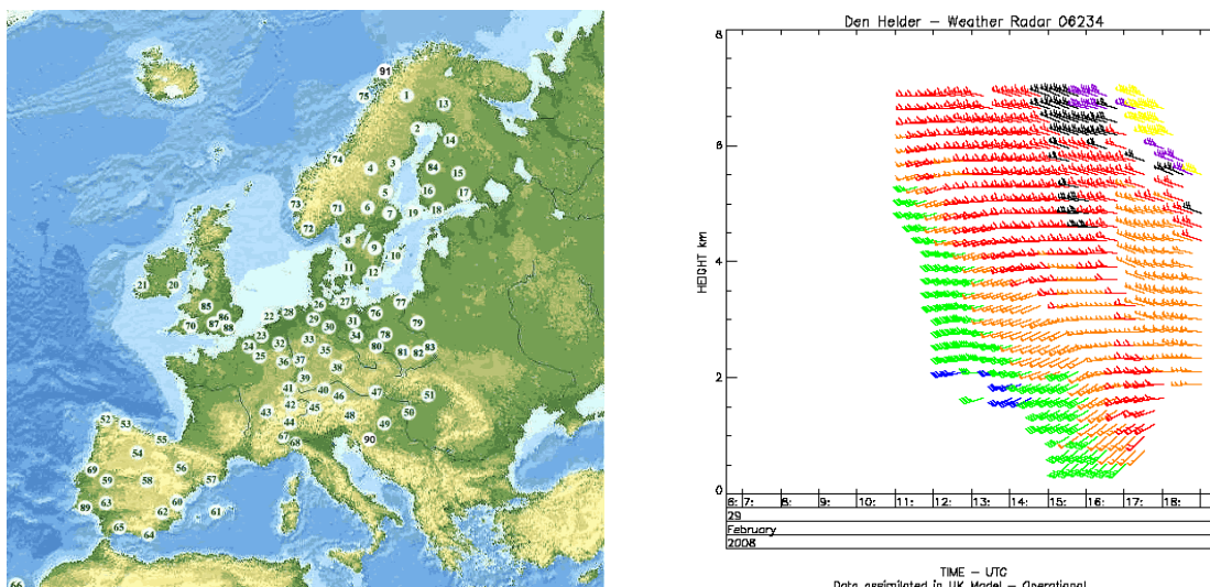
Figure 3. Map in left frame shows the 91 radar sites that are sending profiles in real-time to CWINDE. The right frame shows an example of the display of WRWP on the CWINDE internet site for the KNMI weather radar in Den Helder.
