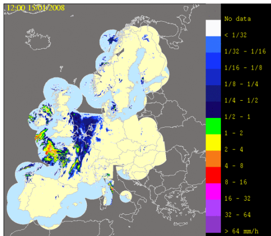
Figure 4. Example of European radar composite from pilot data hub of 15 January 2008 at 1200 UTC.
