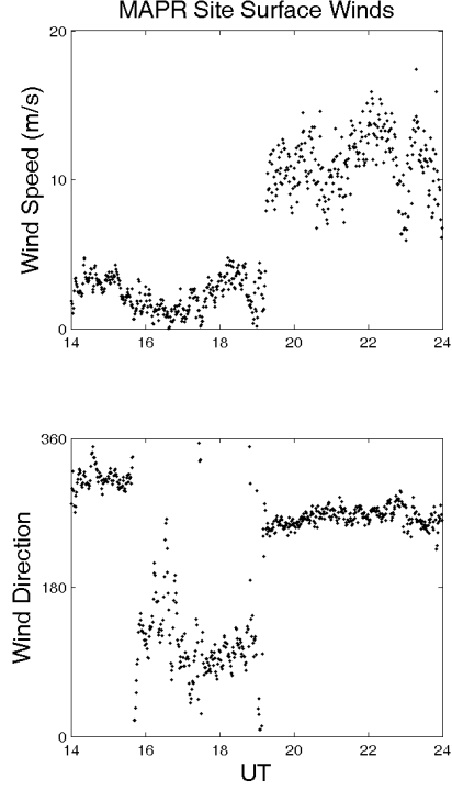
Figure 3: Surface wind speed and direction at the MAPR site from 14-24 UT on March 9, 2006.
