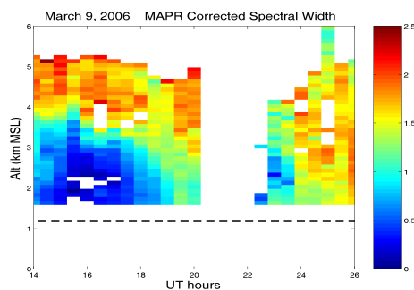
Figure 5: Time-height plot of corrected spectral width from MAPR. Data from 20-22 UT is unavailable due to a power outage.
