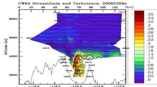
Figure 6: Streamlines and turbulence from the Univ. of Wyoming King Air flight (first T-REX IOP 3 flight on March 9, 2006). Turbulence (EDR, proportional to the cube root of eddy dissipation rate) is colored.
