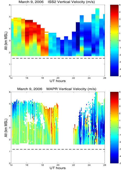
Figure 4: Time-height plot of vertical wind measured with the western-most ISS wind profiler on the valley's alluvial slope (top) and with the eastern-most wind profiler (MAPR) near the center of the valley (bottom). Areas of white are low signal strength or below the first sample height of the profiler. MAPR data from 20-22 UT is unavailable due to a power outage.
